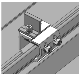
Install with Cross Connector Clamp of ECO-Rail
