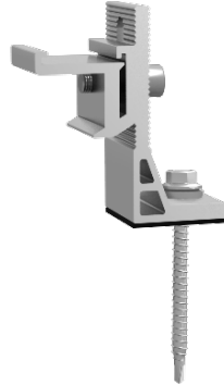
Tin Interface A with ezClick connection for ECO-Rail Part Number: ER-I-05A/EZC/ECO
